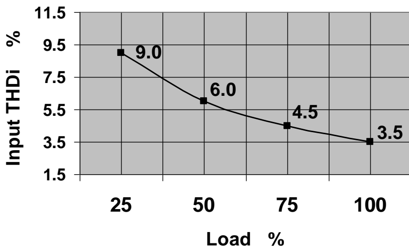
Input Current Distortion THDi
