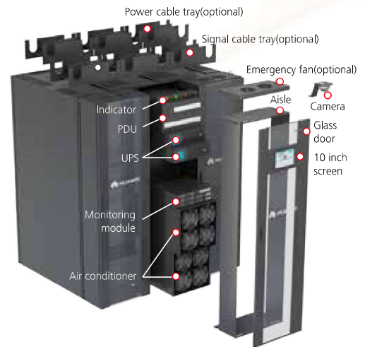
FusionModule800 Architecture
